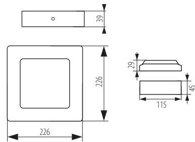
KANTI N LED 18W
