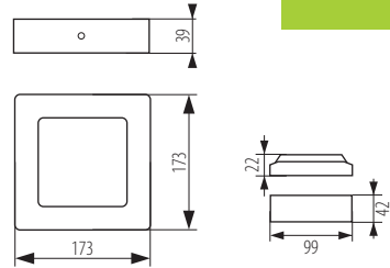
KANTI N LED 12W
