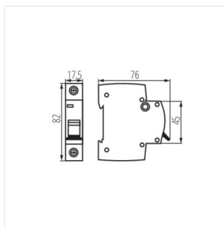
KMB6-B16/1
