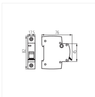
KMB6-B40/1
